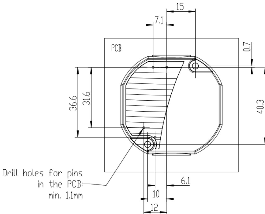
TOP VIEW - pins are on bottom side
